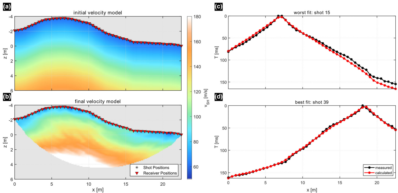
FIGURE 3 Initial (a) and final (b) velocity models of the applied FATT. On the right, a comparison between the measured (black dots) and the calculated (red dots) first arrival times is shown for the worst (c) and best (d) fitting shots. Z = 0 m equals NN, positive values denote a depth below NN.
